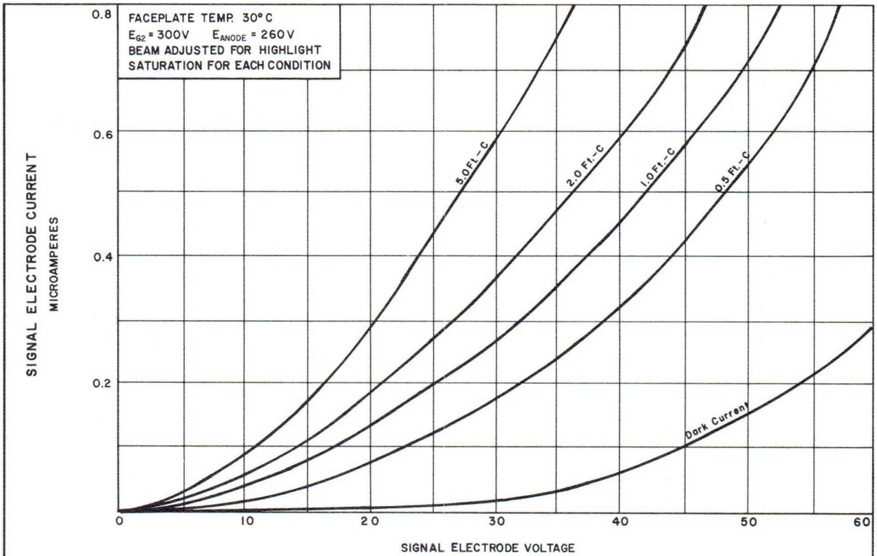
FIG. 5 SIGNAL ELECTRODE VOLTAGE - CURRENT CHARACTERISTICS
