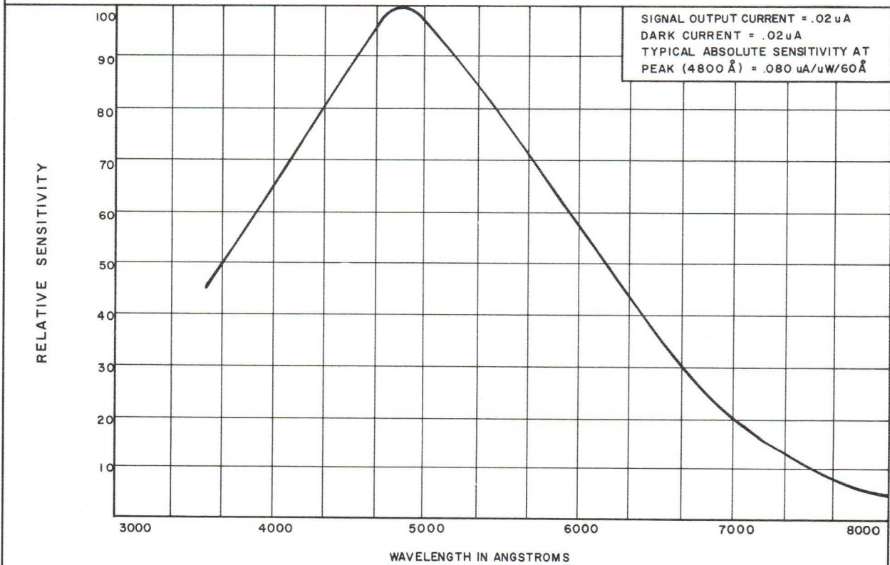
FIG. 4 SPECTRAL RESPONSE
