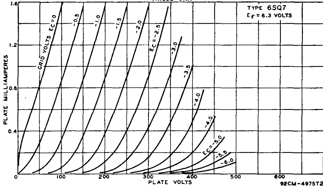
AVERAGE PLATE CHARACTERISTICS TRIODE UNIT
