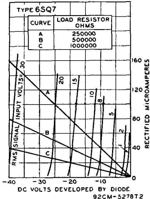
AVERAGE CHARACTERISTICS HALF-WAVE RECTIFICATION-SINGLE DIODE UNIT
