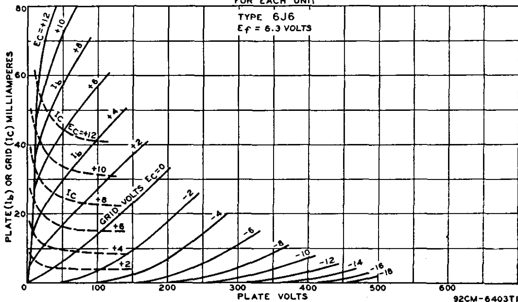
AVERAGE PLATE CHARACTERISTICS FOR EACH UNIT
