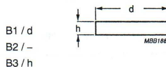
Fig.4 D Discs/Rods (axial).
