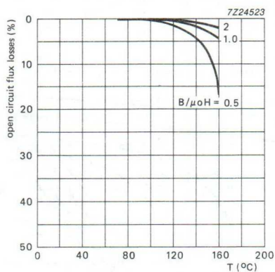
Fig.3 Open circuit irreversible losses as a function of temperature for RES 255.
