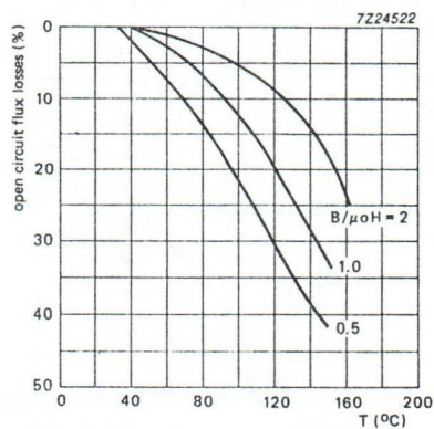
Fig.3 Open circuit irreversible losses as a function of temperature for RES 300.
