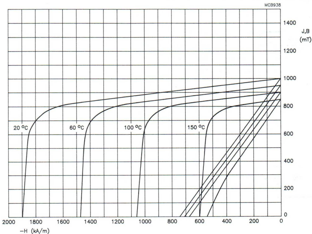
Fig.2 Demagnetization curves for Neodure RES 257 at several temperatures.
