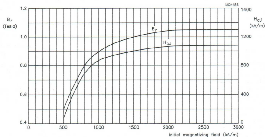
Fig.3 Magnetizing field dependence of Neodure RES 270.
