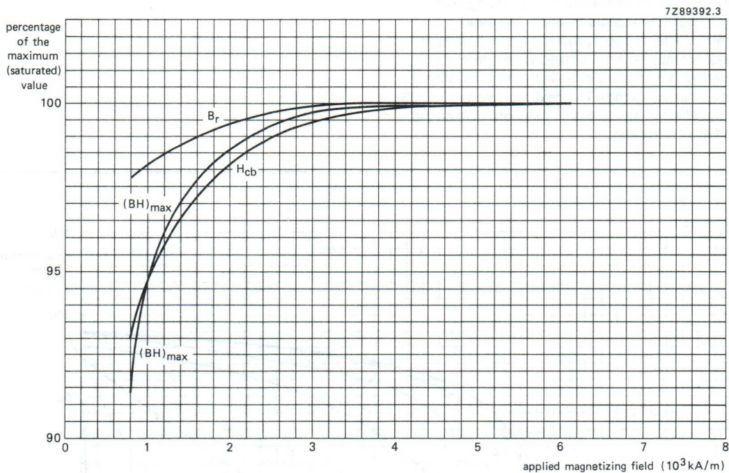
Fig.3 B_r , H_{cb} and (BH)_{max} as a percentage of the maximum obtained (saturated) value as a function of magnetizing field strength. Values are typical for a RES 190 magnet not previously magnetized.
