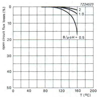
Fig.3 Open circuit irreversible losses as a function of temperature for RES 305.
