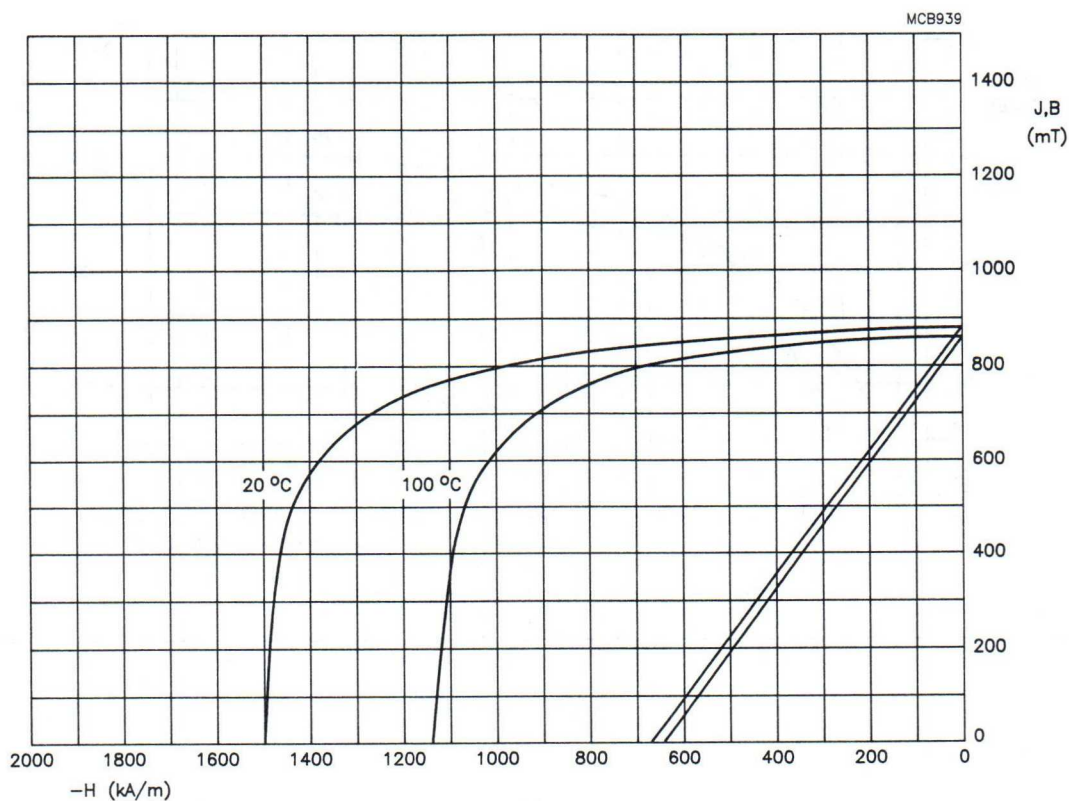
Fig.2 Demagnetization curves for RES 195 at several temperatures.
