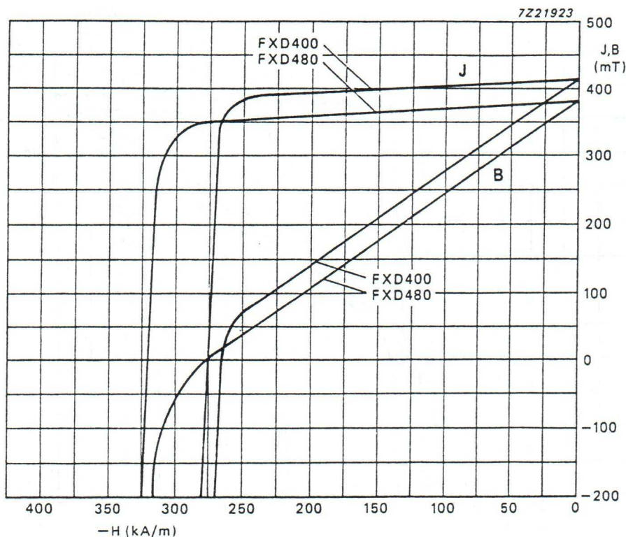
Fig.6 Typical demagnetization curves, Ferroxdure 400 series.
