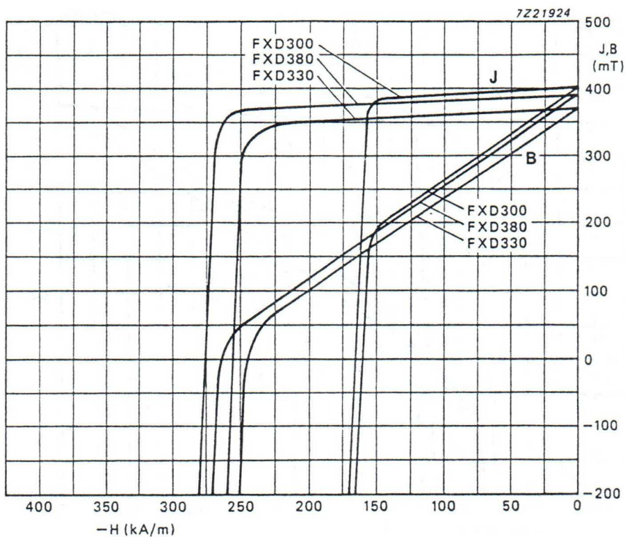
Fig.5 Typical demagnetization curves, Ferroxdure 300 series.
