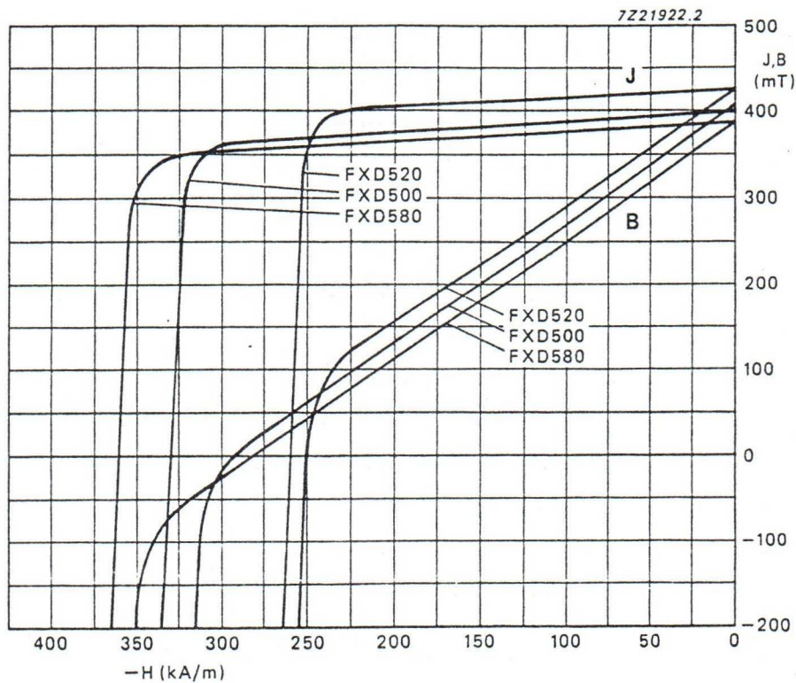
Fig.7 Typical demagnetization curves, Ferroxdure 500 series.
