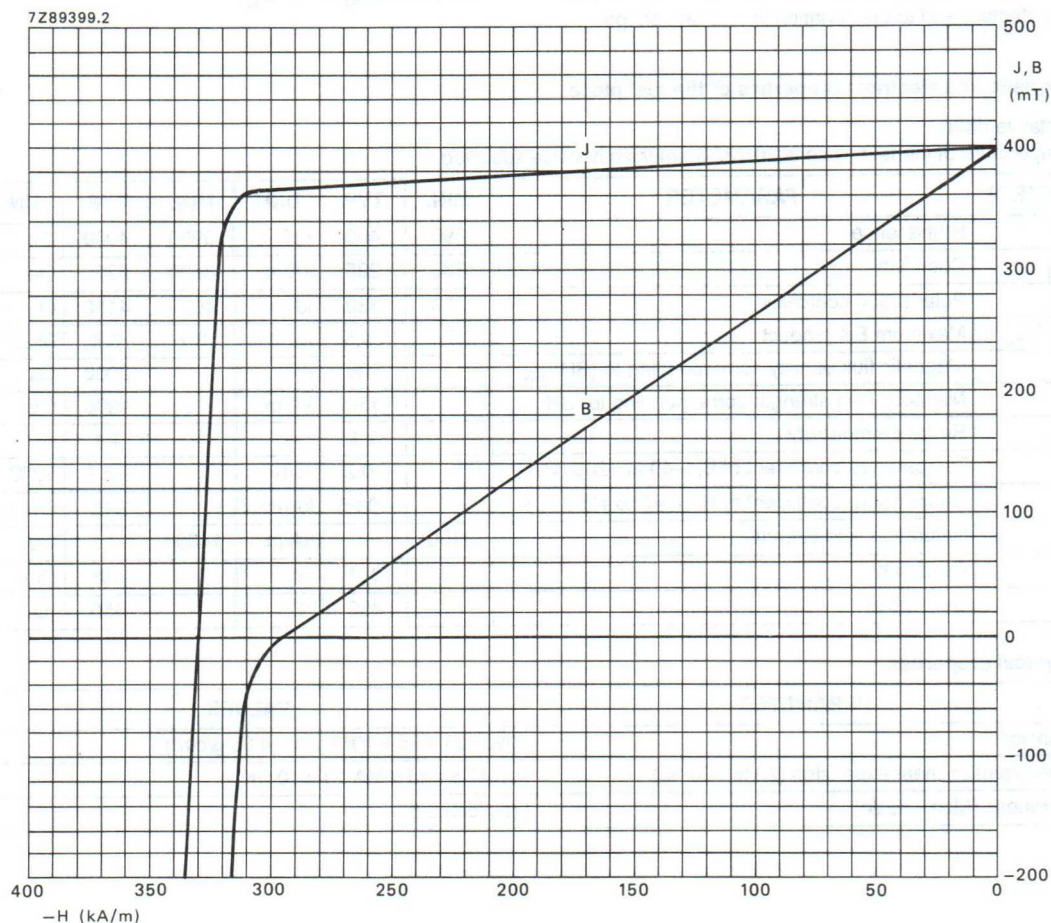
Fig.1 Typical demagnetization curve (20 °C) FXD 500.
