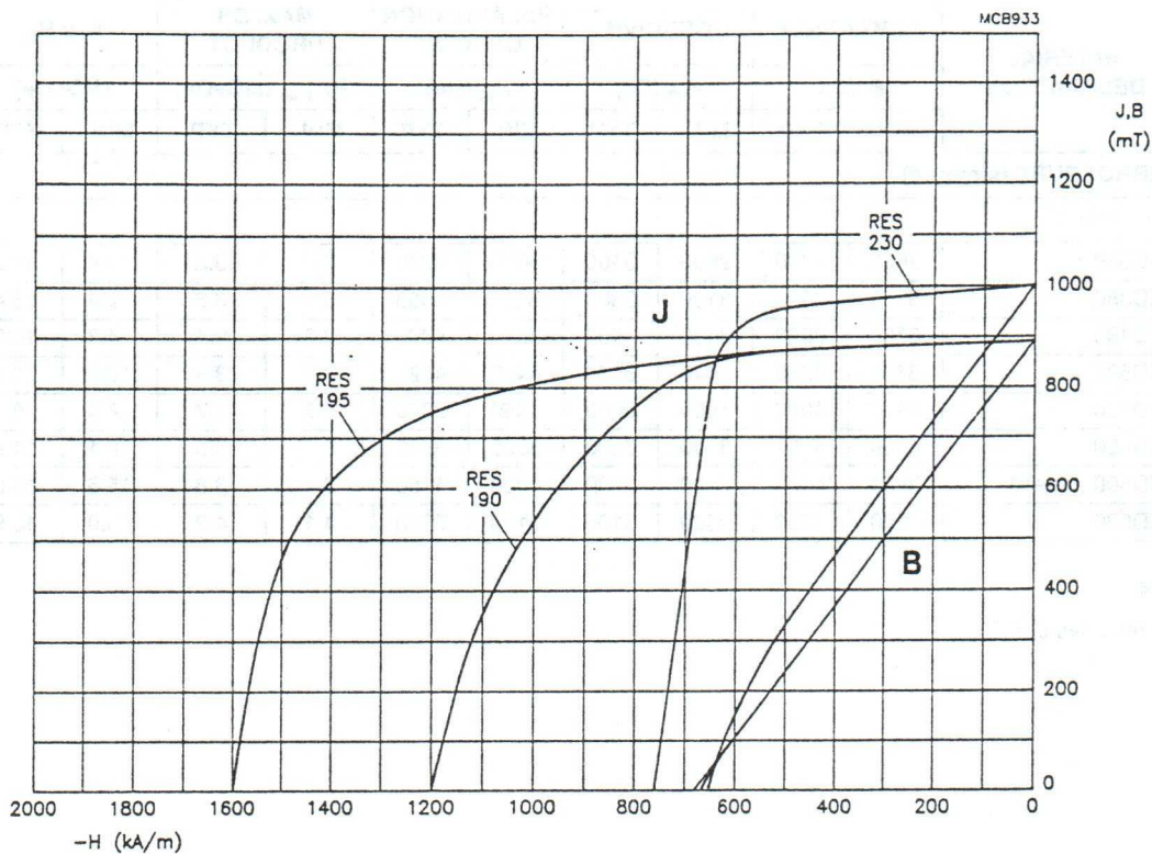
Fig.2 Typical demagnetization curves, Samarium Cobalt grades.
