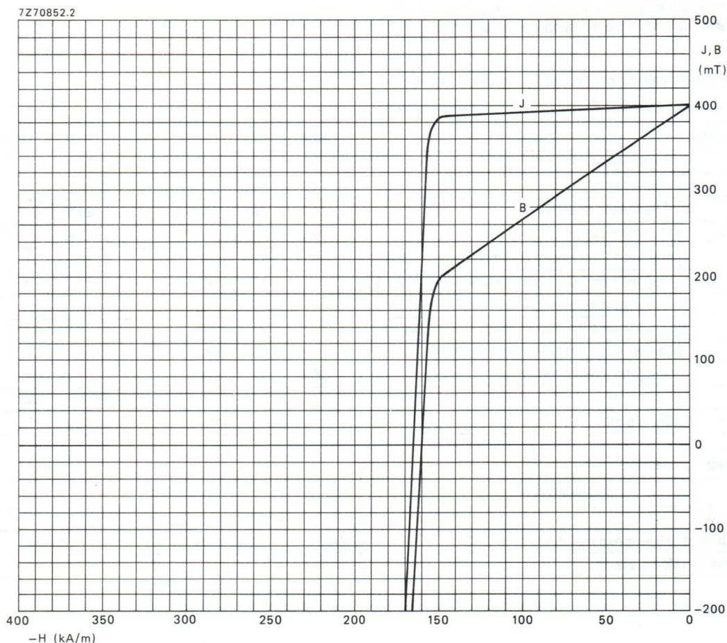
Fig.1 Typical demagnetization curve (20 °C) FXD 300.
