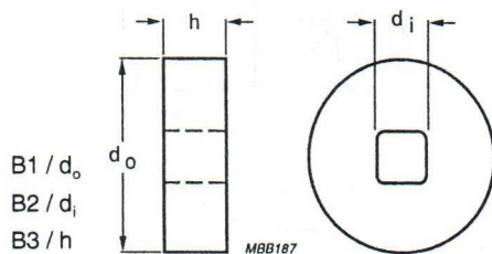
Fig.3 R Rings/Cylinders (axial).
