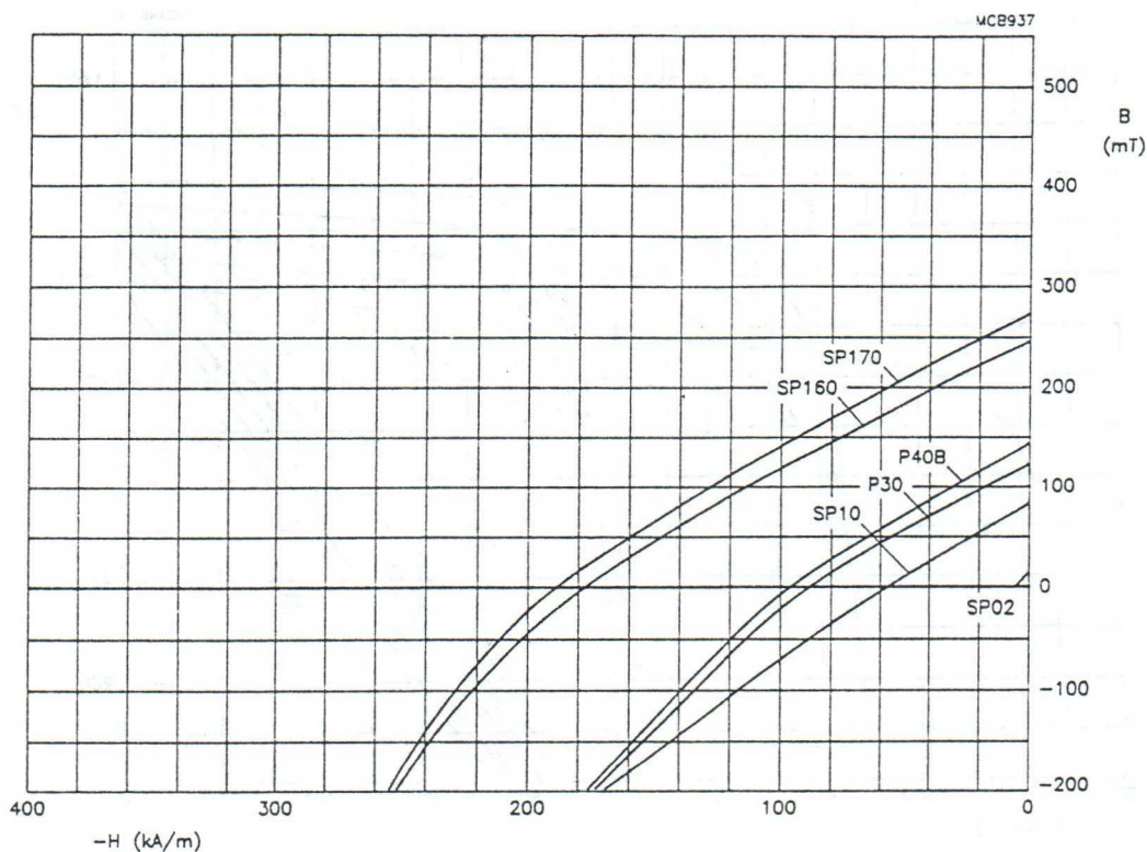
Fig.4 Typical demagnetization curves, Plastic-bonded ferroxdure.
