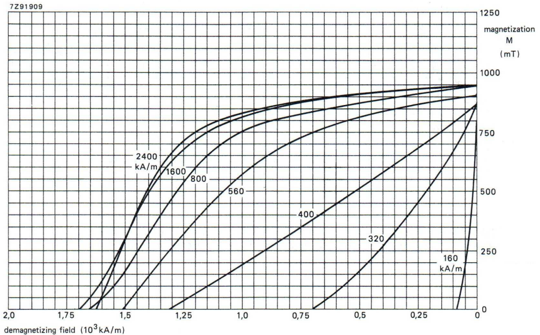
Fig.2 Thermally demagnetized RES 190 magnets; dependence of coercivity on initial magnetizing field.
