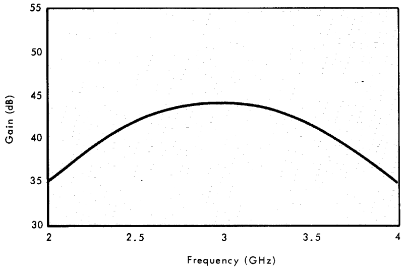
SATURATED GAIN
