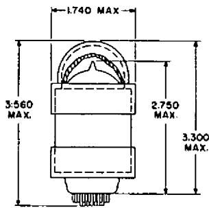
FIG. 1. OUTLINE DRAWING
